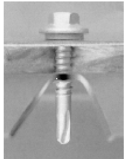
Maxiseal Head
